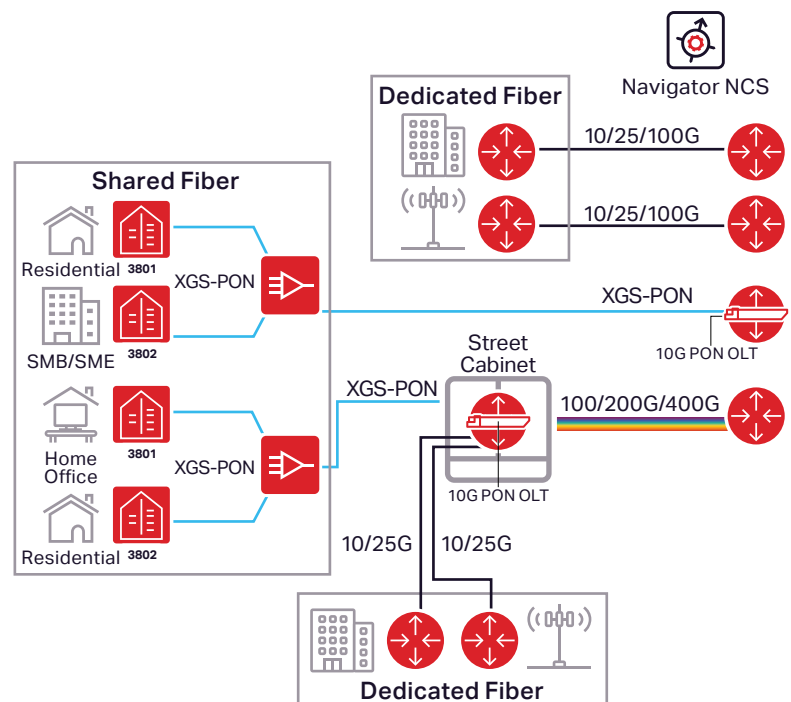
Figure 3. PON deployment and universal aggregation
